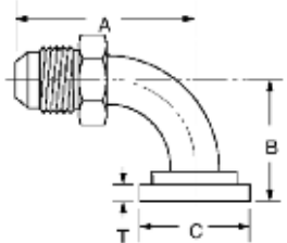
90° Elbow
