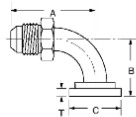
90° Elbow
